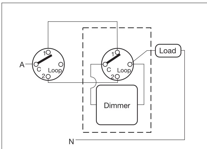
Fig 3. Two-way wiring diagram
