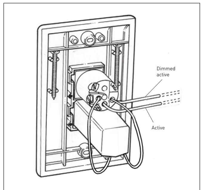
Fig 1. View from back of plate
