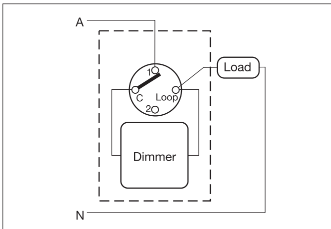
Fig 2. One-way wiring diagram
